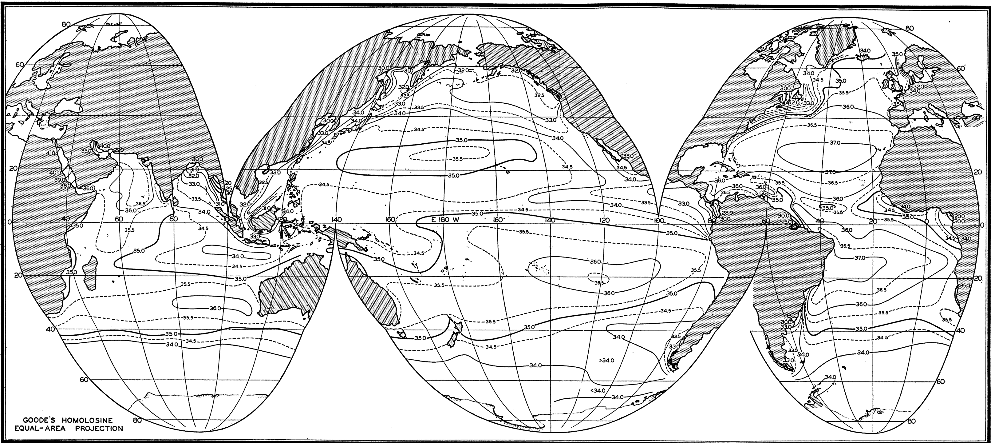
Chart VI. Surface salinity of the oceans in northern summer.
