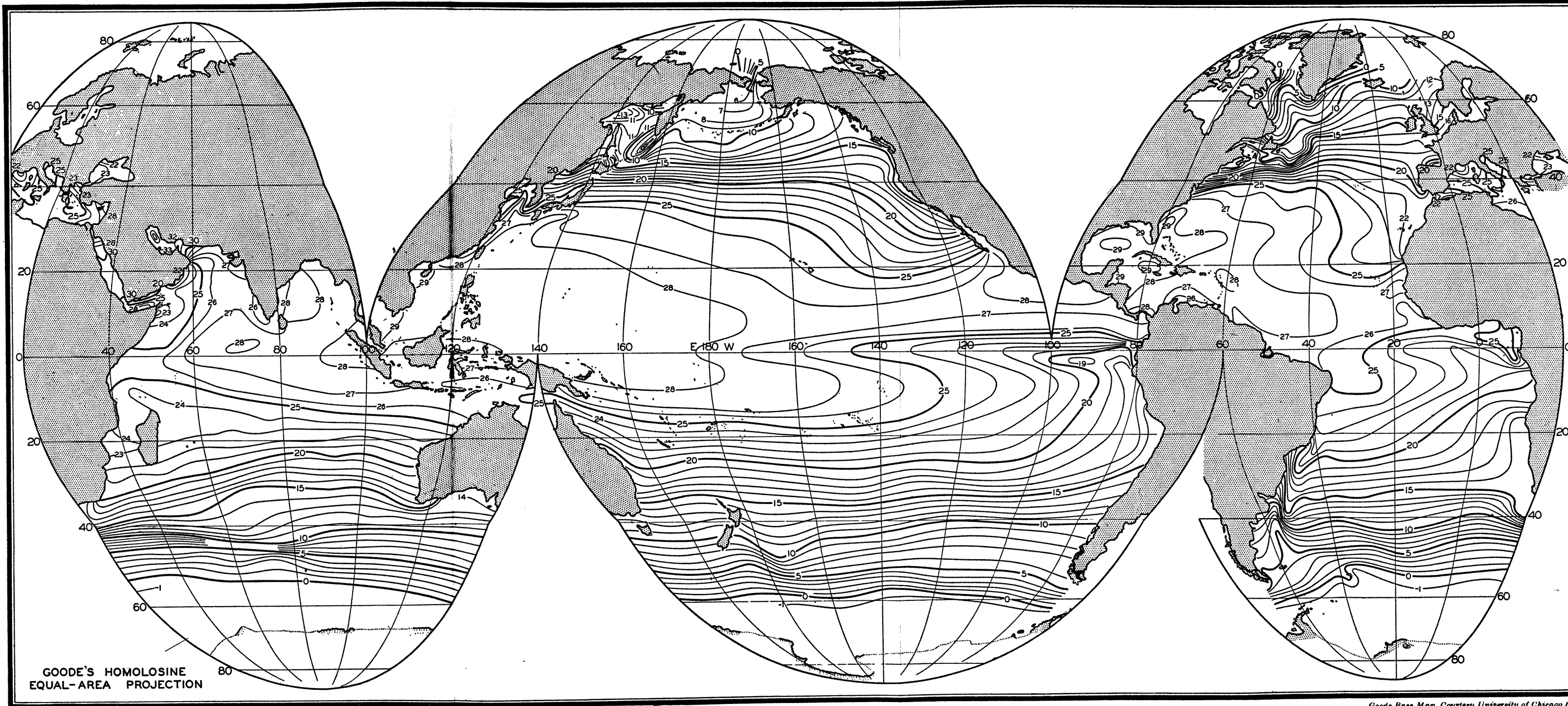
Chart III. Surface temperature of the oceans in August.
