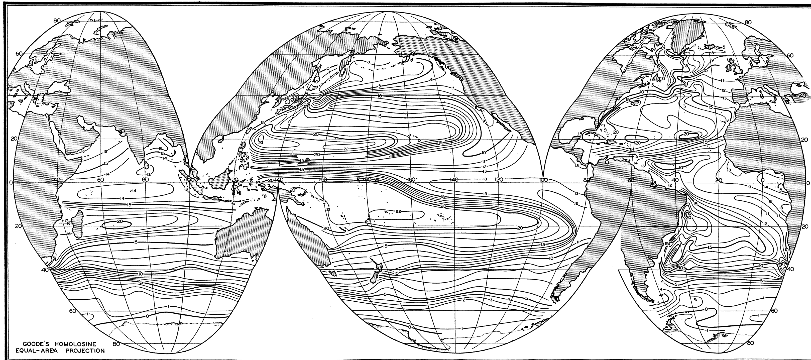
Chart IV. Temperature of the oceans at a depth of 200 meters.
