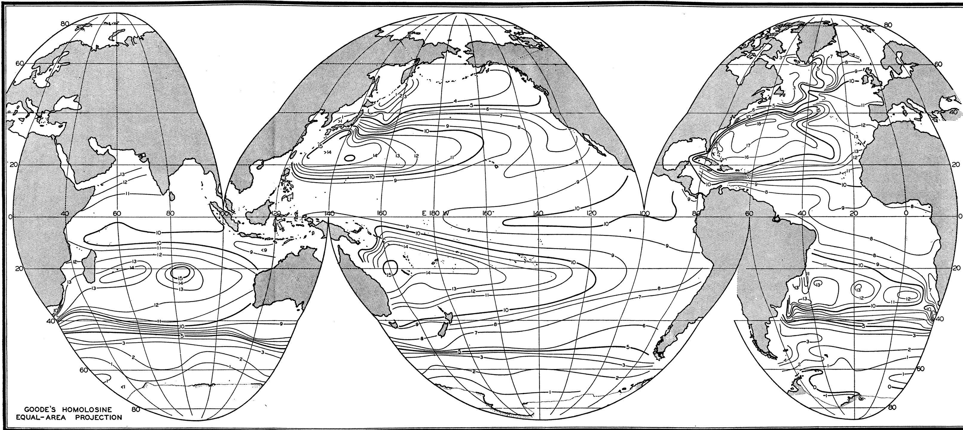
Chart V. Temperature of the oceans at a depth of 400 meters.
