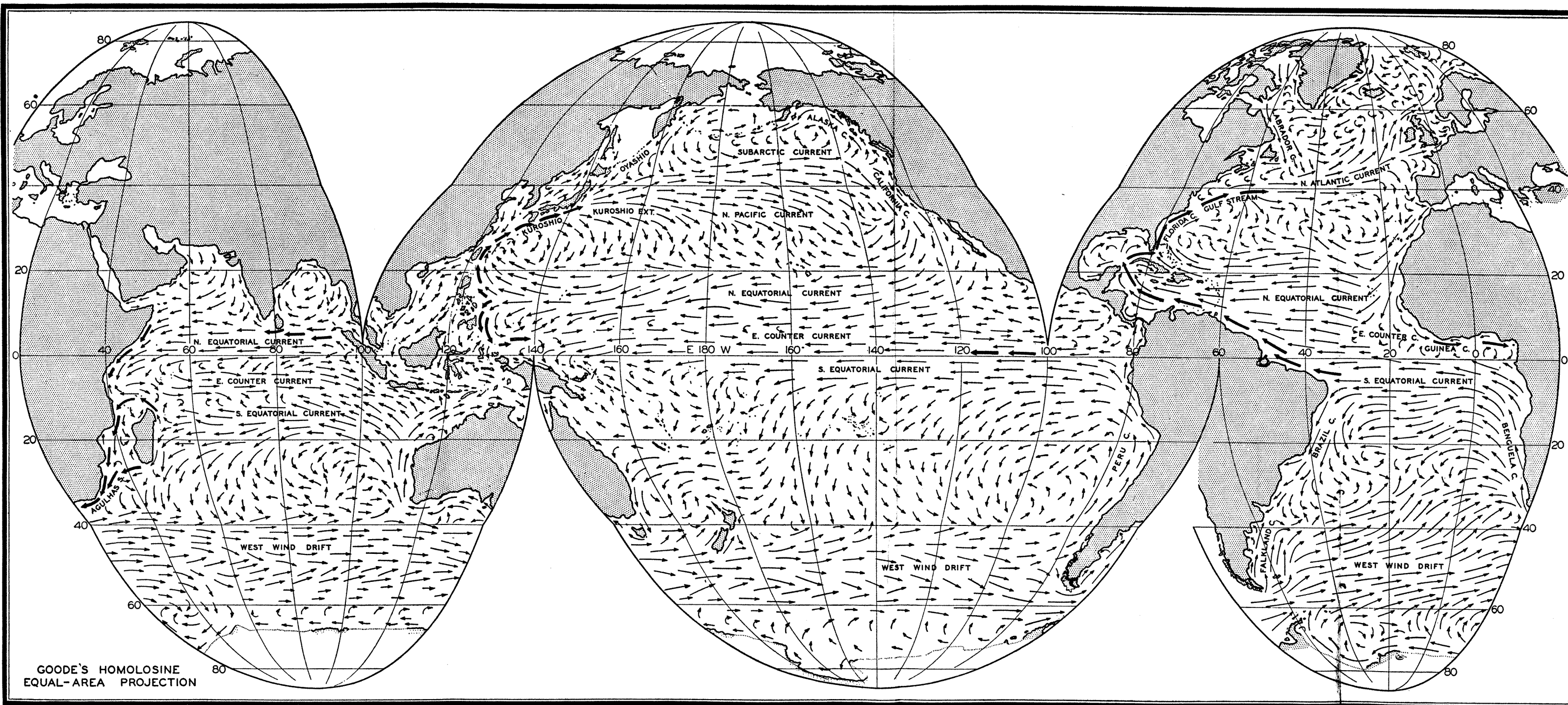
Chart VII. Surface currents of the oceans in February-March.
