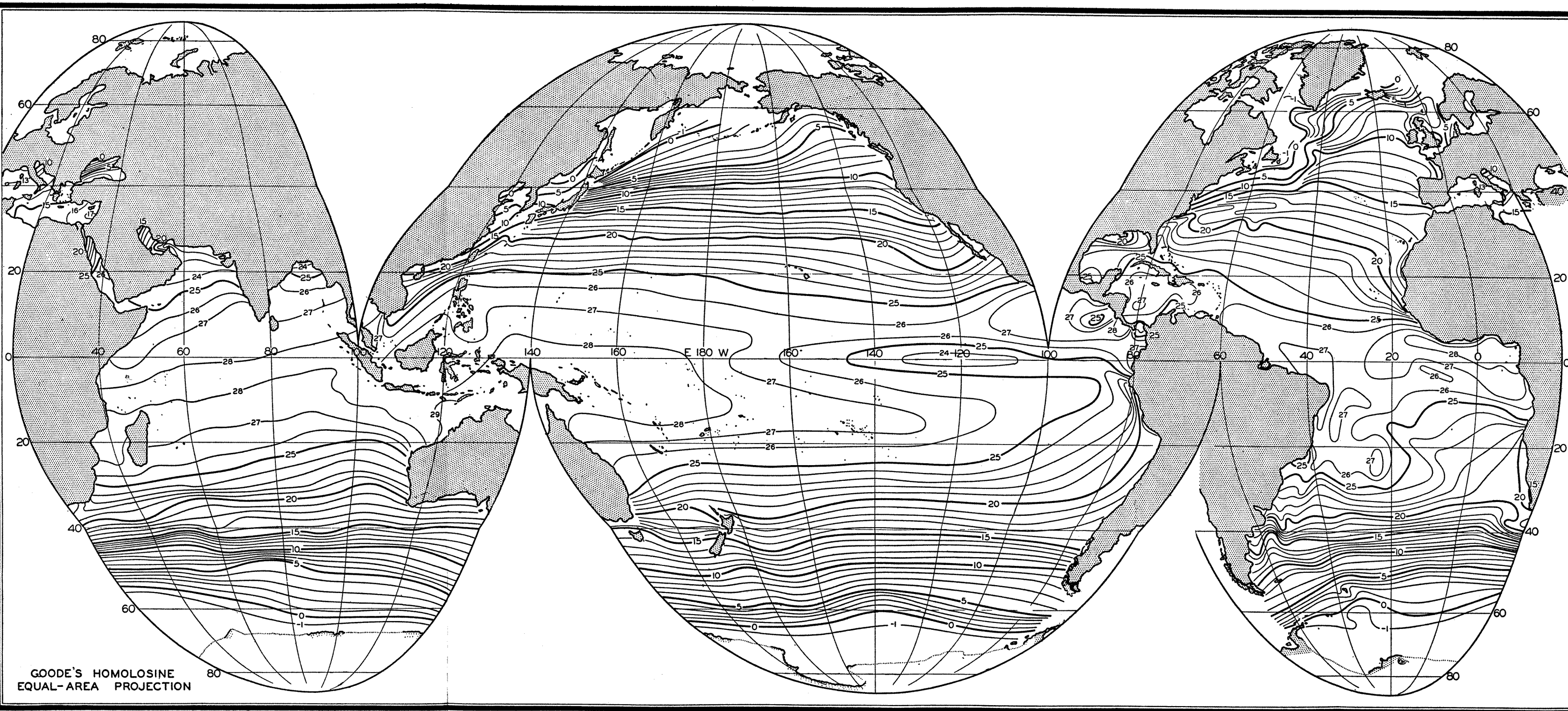
Chart II. Surface temperature of the oceans in February.
